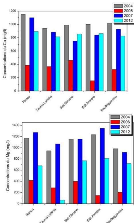
Figure 2: Variation spatio-temporelle des cations
