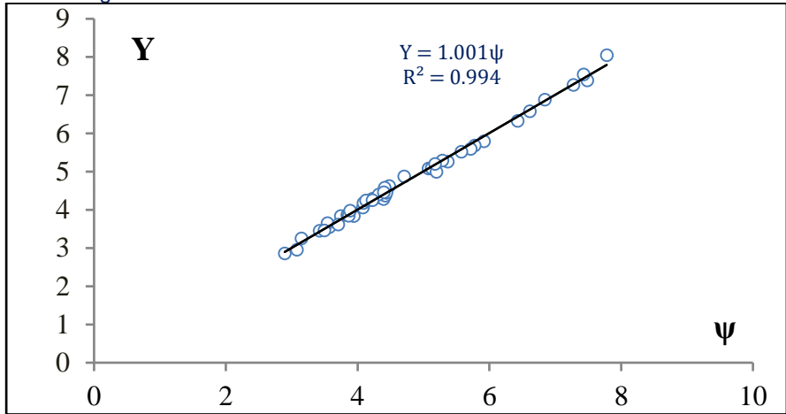
Fig.II. Variation of Y = h_2 / h_1 as a function of \psi = (-0,139\gamma + 1, 09) F_1 . (o) Experimental points. (-) line of equation: h_2 / h_1 = (-0,139\gamma + 1, 09) .F_1
