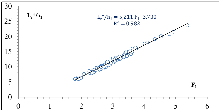
Fig.8. variation of L_r^*/h_1 as a function of the inflow Froude number F_1 ,
