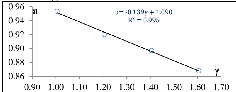
Fig.10. Variation of the coefficient ( a ) as a function of the ratio \gamma of Compactness. (-) adjustment curve.
