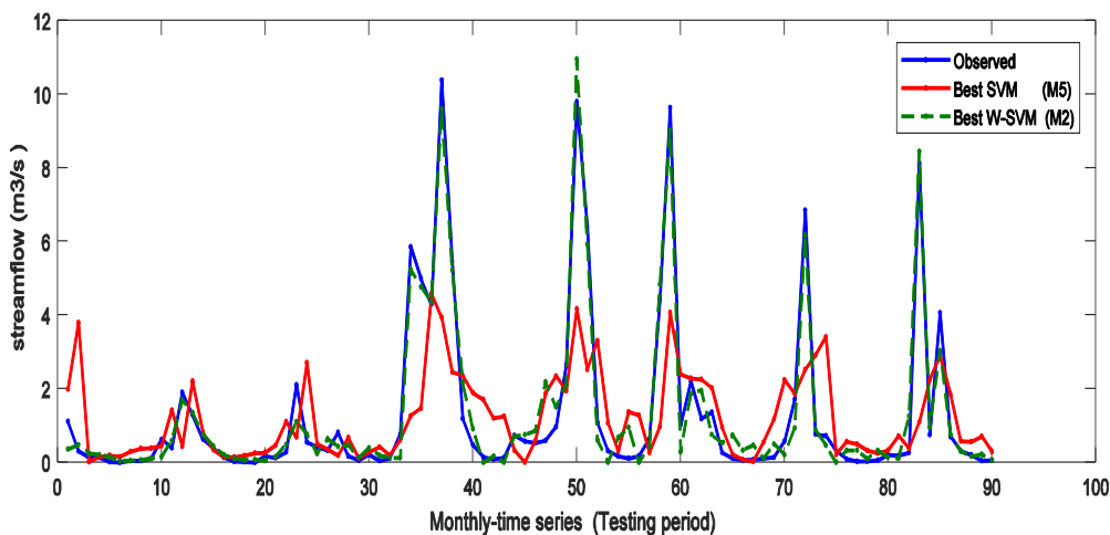
Fig. 1 - Best performance of the SVM and W-SVM models versus observed values in the testing period.
