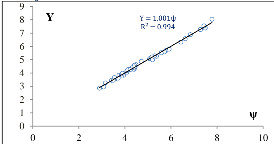
Fig.11. Variation of Y = h_2 / h_1 as a function of \psi = (-0,139\gamma + 1,09) F_1 . (o) Experimental points. (-) line of equation: h_2 / h_1 = (-0,139\gamma + 1,09) .F_1
