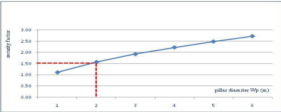
Fig. 2 - Relation between the safety factor and the deffernet pillars diamiter.
