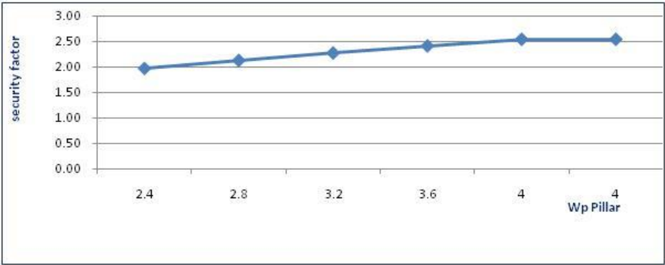
Fig. 1 - The relation between the safety factor and the actual dimensions of the pillars.
