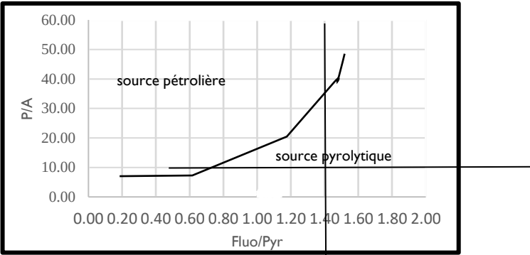
Figure 2 : Double ratio P/A = fn (Fluo/Pyr) [11].
