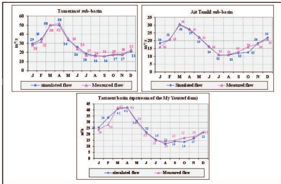
Fig. 5. Comparison of measured and simulated flows on a monthly scale (1986-2010)
