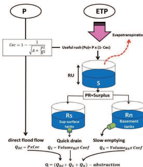
Fig. 2. Architecture of the Orchy II hydrological model in the Tassaout basin (upstream of the Moulay Youssef dam).
